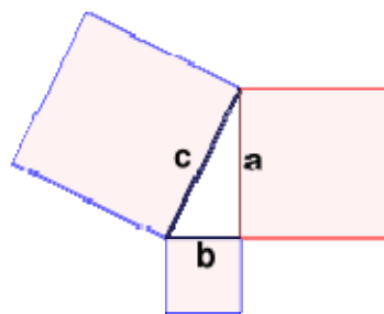
The Pythagorean theorem
